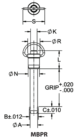
Ring Handle (R)
