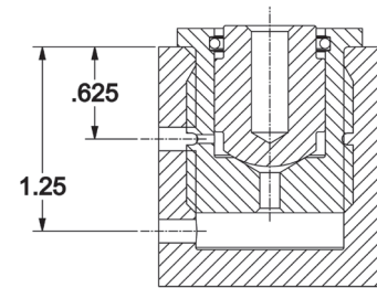
Air connection with drilled manifold passage
