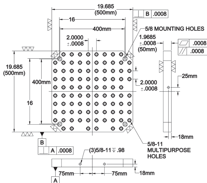
JIS Mounting
