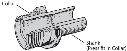
ADAPTOR TIP ASSEMBLY
