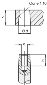
Standard clamping arm
