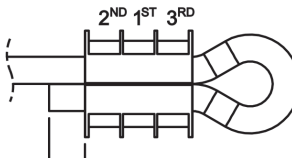
Cable #3 Three Crimps (Sequence Option 2)
