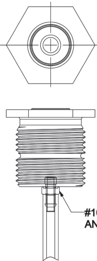
Air connection with external fitting
