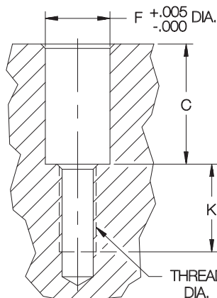
Installation Hole
