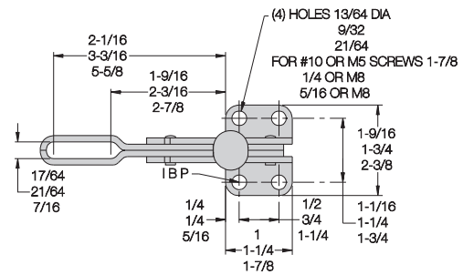
CL-11-TC
