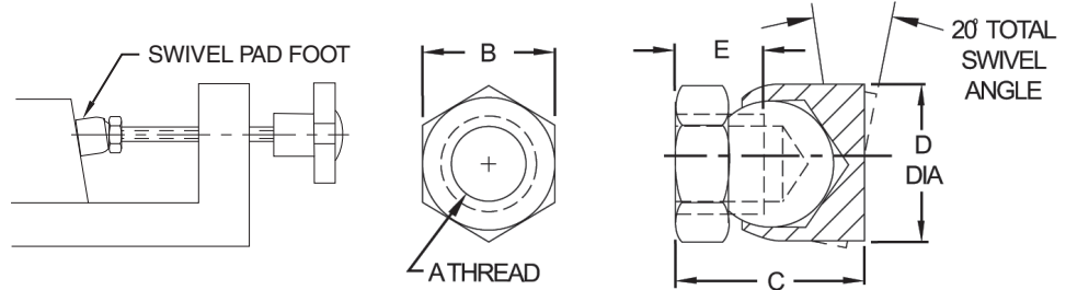
Steel Zinc Plated with Delrin® Pad
