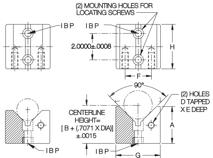
Standard—Small V
