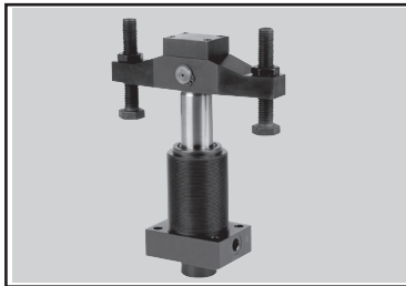
B1.8802 Swing Clamps with Reinforced Swing Mechanism 160 bar
