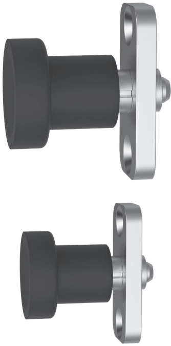
Knob Handle with Mounting Plate (Locking Type)
