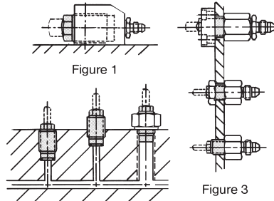
Figure 1 Figure 2 Figure 3 Mounting Options
