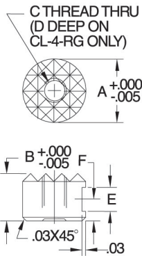
Hardened Tool Steel (Serrated)
