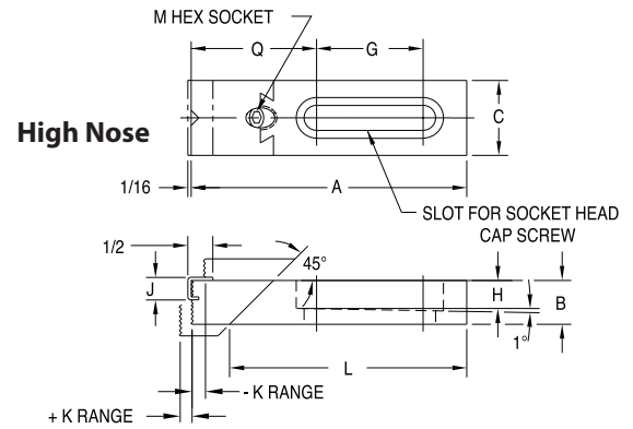
Serrated Adjustable Edge Clamp (High Nose)
