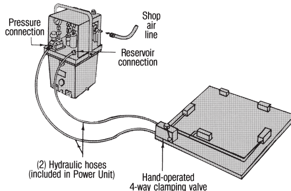
Single Fixture Double Acting CLR-103-AP
