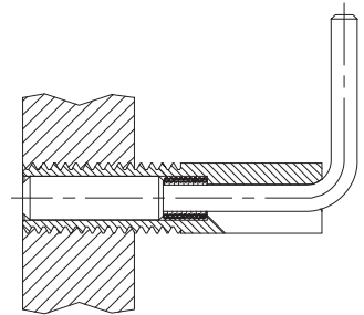
Retracted Position
