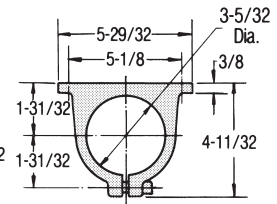
Foot Lever CLR-002-HPA
