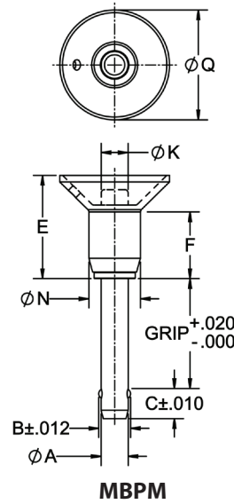
Recessed Button Handle (M)
