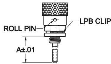
ASSEMBLY EXAMPLE
