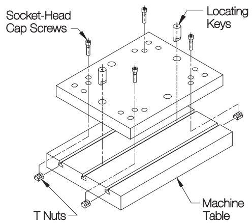
T-Slotted Table
