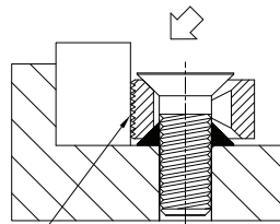
SERRATED JAW
