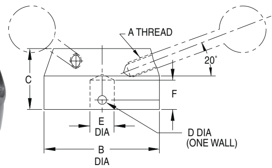
Triple Hub
