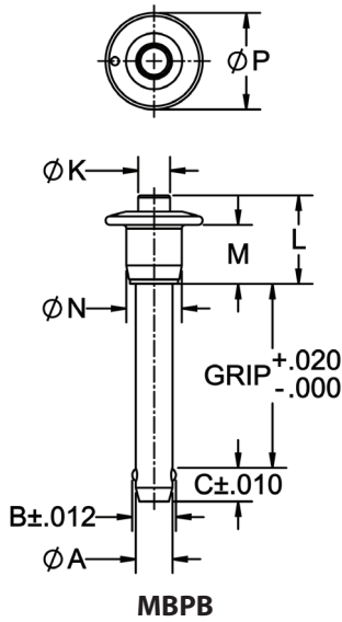
Button Handle (B)
