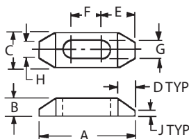
Plain Clamp
