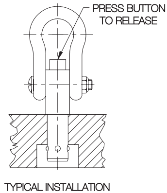
TYPICAL INSTALLATION
