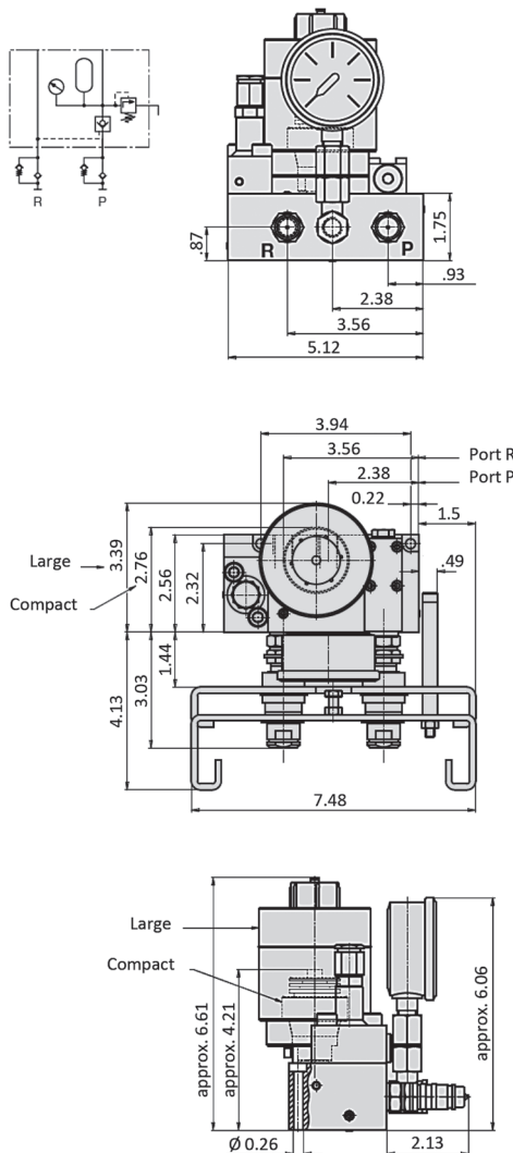
Single Acting or Double Acting with Automatic Shutoff
