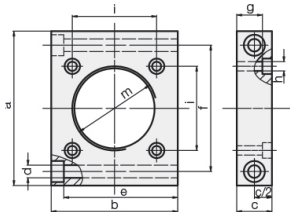
Threaded nut
