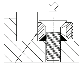
SMOOTH JAW
