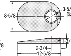
Weighted Base CLR-301-HPA
