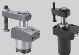
Top Flange pages 617-618
