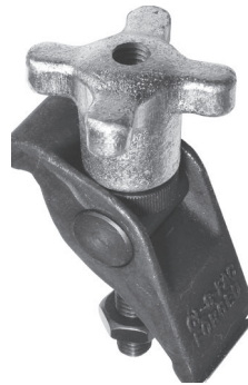
Assembly with Hand Knob CL-x-FACA-HK
