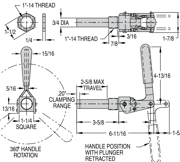
CL-355-TPC
