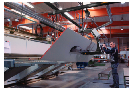
The sheet gripper is ideal for handling sheets of wood. Add a tilting function and you can easily tilt loads of up to 250 kilos, up to 180 degrees.
