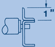
Angle Type Guardrail: 1" x 1" x 1/8" Steel
